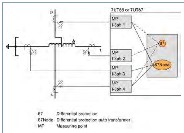
Figure 3.2/22 Protection of an Auto-Transformer Bank by 2 Differential Protection Functions in one Device
