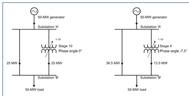
Figure 3.2/23 Power Distribution between 2 Lines when Using Different Phase-Angle Values
